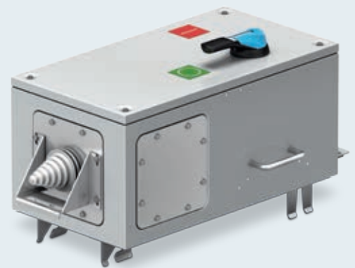
Tap-off unit with fuse-type switching device
